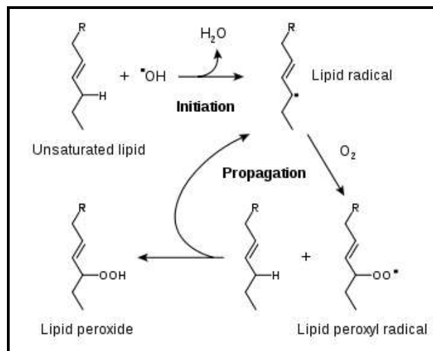
Figure 1: Oxidation process of fatty acids
